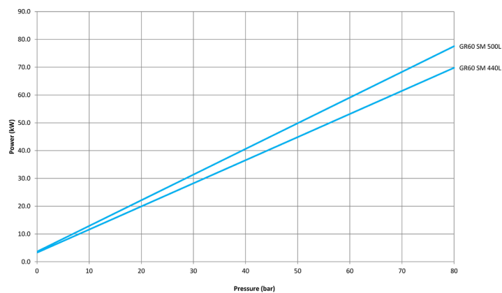
Power GR60 SM @ 2750 RPM - 68 cSt
