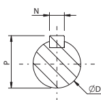
Shaft dimensions
