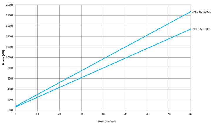
Power GR80 SM @ 2750 RPM - 68 cSt
