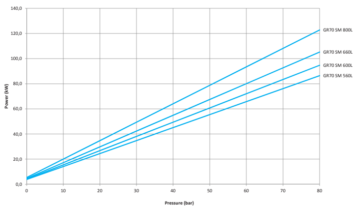
Power GR70 SM @ 2750 RPM - 68 cSt
